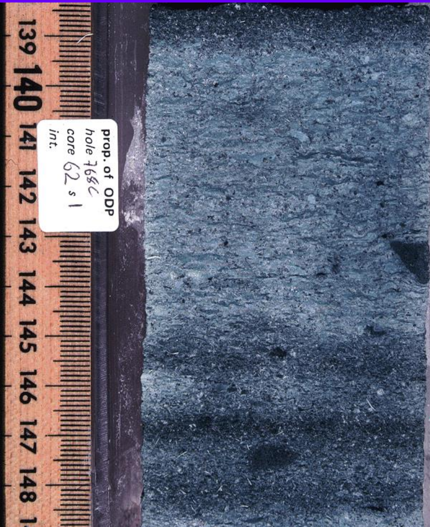
Back arc basins
