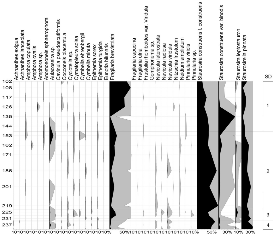
Fig. 6. – Diagram of relative frequency of occurrence of diatoms in the Šúr profile.
