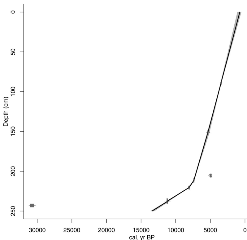
Fig. 3. – Depth-age model of the Šúr profile based on linear interpolation between dated levels based on estimated sedimentation rates. Cross indicates assumed outlying dates (UG-5590, UG-5392 and UG-5393).
