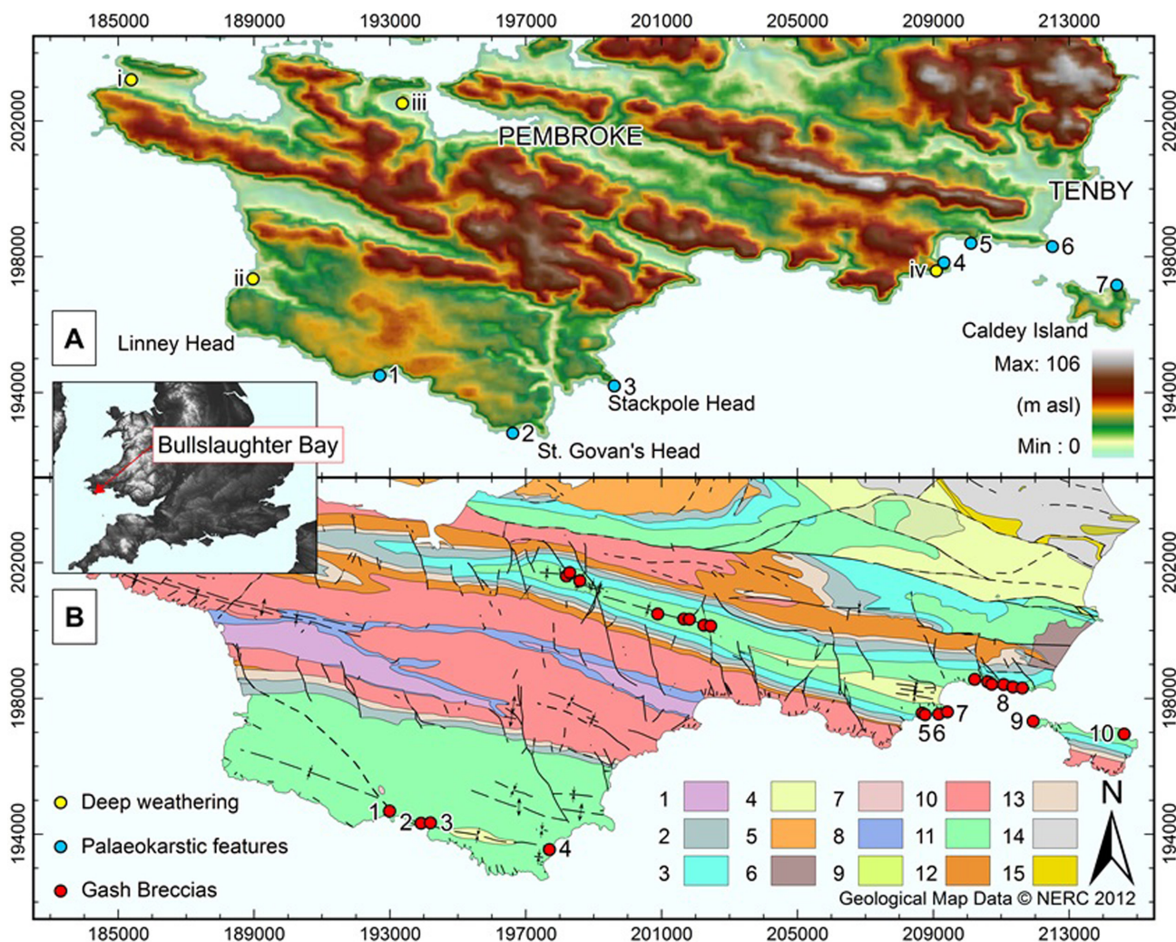
Figure 1. (A) The topography of southern Pembrokeshire constructed using SRTM data from the CGIAR-CSI GeoPortal ( srtm.csi.cgiar.org ). The yellow dots represent the location of potentially analogous weathering sites (i: West Angle; ii: Pole Reef Cove; iii: Pembroke Power Station; iv: Lydstep Mine) while the blue dots represent the location of palaeokarstic sites (1: Elegy Stacks; 2: St. Govan's Chapel; 3: Stackpole Head; 4: Lydstep Cleft; 5: Proud Giltar; 6: Giltar Point; 7: Highcliff Quarry). (B) The regional geology constructed using data from the British Geological Survey (1: Aber Mawr Shale Fm.; 2: Avon Group; 3: Black Rock Subgroup & Oolite Fm.; 4: Bishopston Mudstone Fm.; 5: Cosheston Group; 6: Devonian and Carboniferous (undifferentiated); 7: Palaeogene and Neogene (undifferentiated); 8: Ludlow Rocks (undifferentiated); 9: Millstone Grit Group; 10: Milford Haven Group; 11: Pembroke Limestone Group; 12: Ridgeway Conglomerate Fm.; 13: Shrinkle Sandstone Fm.; 14: South Wales Lower Coal Measures Fm.; 15: Telpyn Point Sandstone Fm.). The red dots represent the location of major bodies of Gash Breccia (1: Flimston; 2: Bullslaughter Bay West; 3: Bullslaughter Bay East; 4: Trevalien; 5: Draught; 6: Whitesheet Rock; 7: Lydstep Point; 8: Valleyfield Top; 9: St. Margaret's Point; 10: Den Point) (© Crown Copyright 2013; a British Geological Survey/EDINA supplied service).
